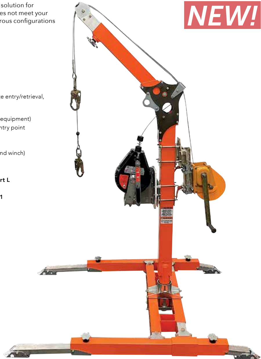
V85043 Davit Arm System
