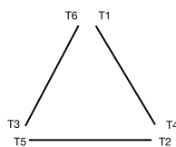
STANDARD 6 LEAD DELTA CONNECTED
