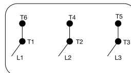
DUAL WINDING FOR PARALLEL INVERTERS DELTA CONNECTED
