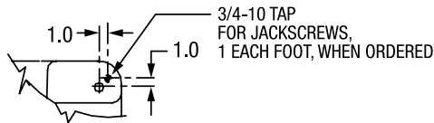
BOTTOM VIEW OF FOOT
