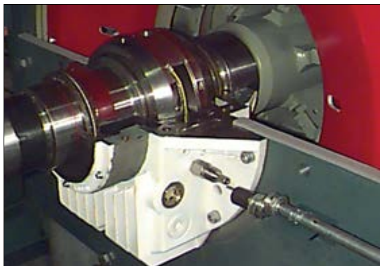
◀ Sleeve Bearing
