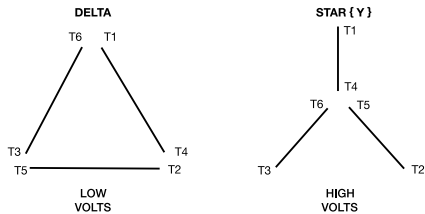
STANDARD 6 LEAD (DELTA / STAR {Y} CONNECTED) DUAL VOLTAGE (LOW VOLTS / HIGH VOLTS)
